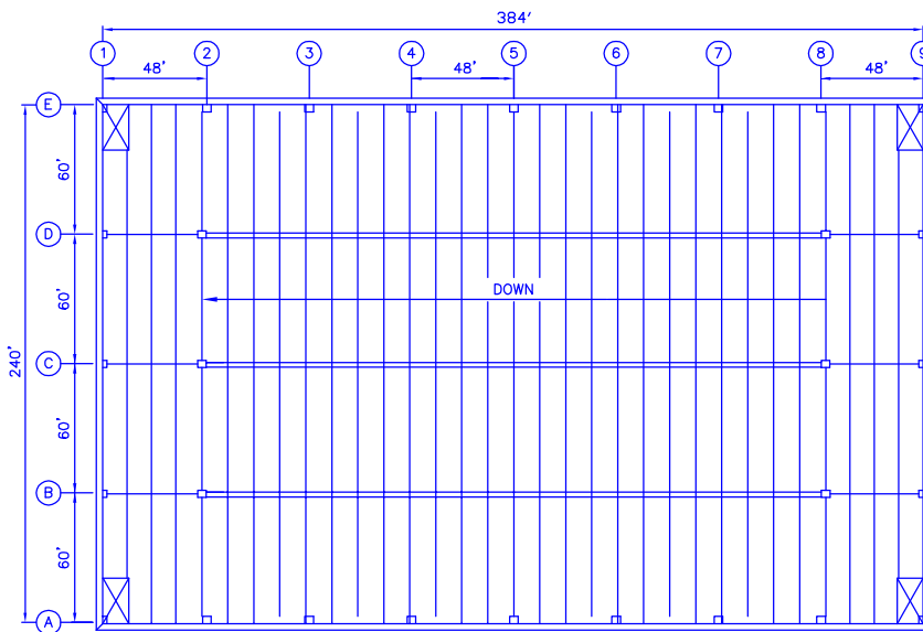
12'-0" DOUBLE TEE LAYOUT
